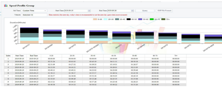
Statistical Analysis of Driving Styles
